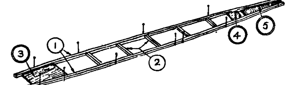
FIG. 1 Longerons (1) pinned down and struts (2) together with pieces 3, 4 and 5 cemented in place.
