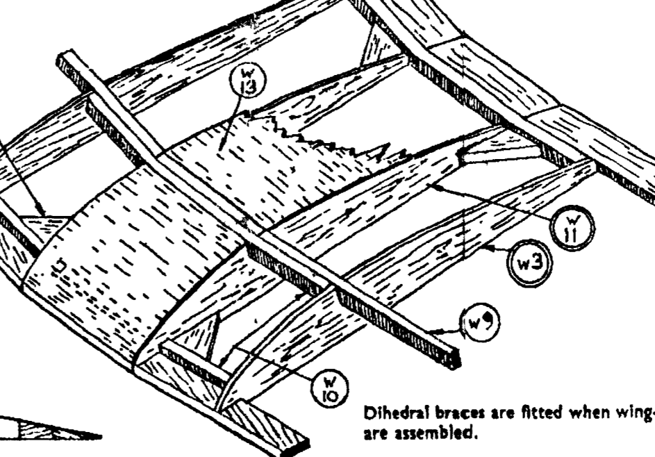
FIG. 5 Wing Centre Section assembly.
