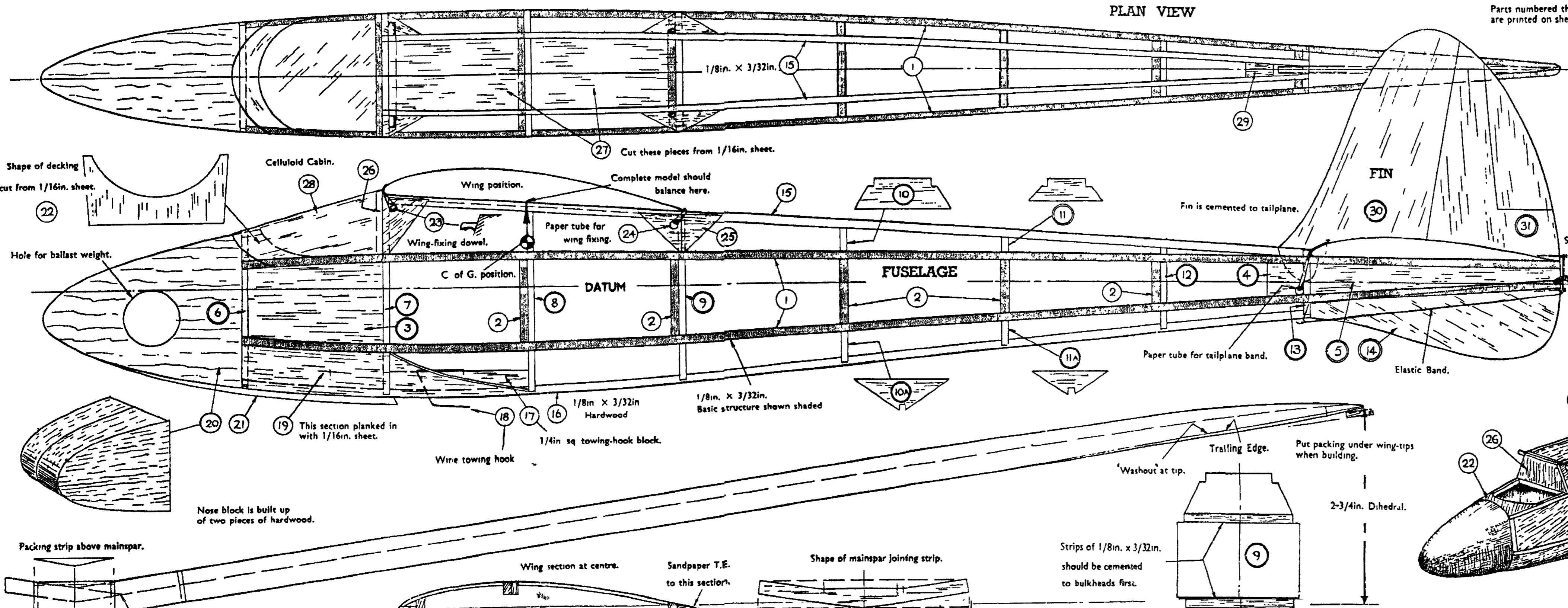
FIG. 1 Longerons (1) pinned down and struts (2) together with pieces 3, 4 and 5 cemented in place.
